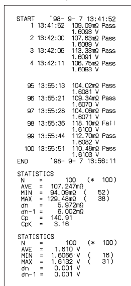
Statistical processing
